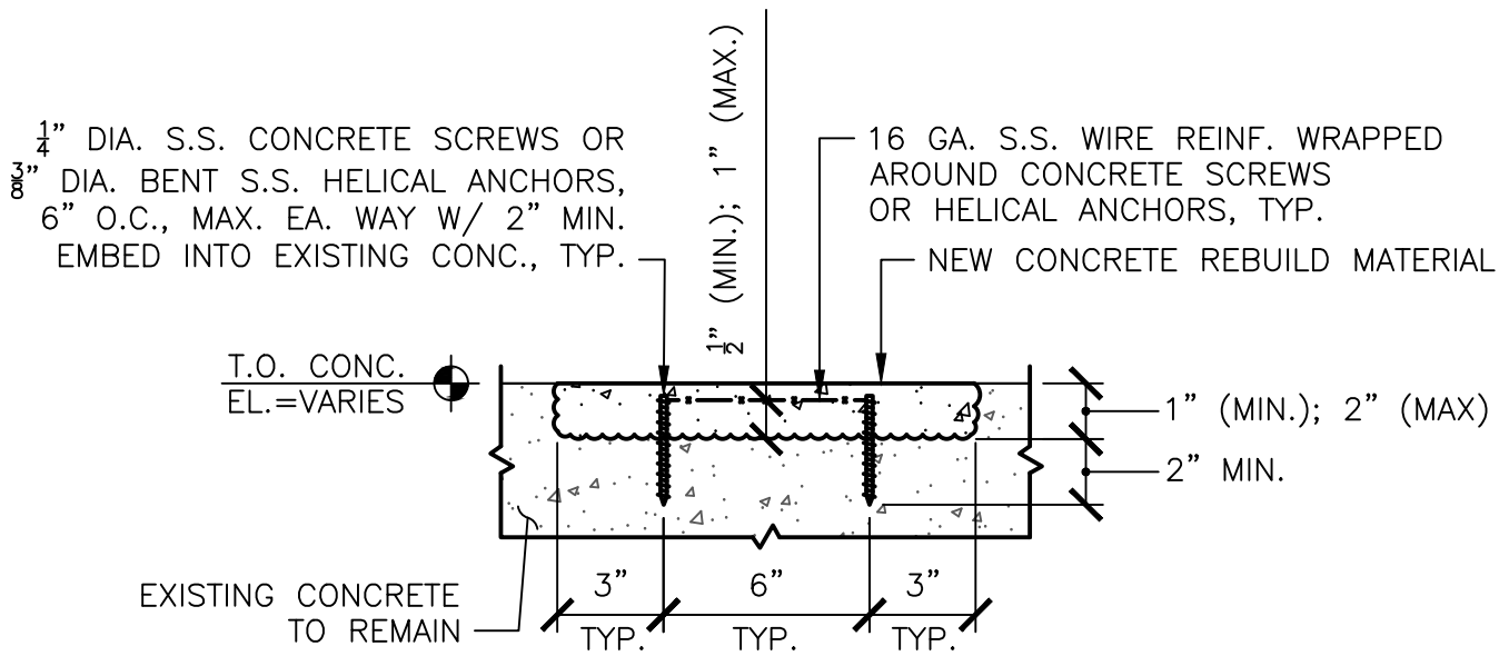
SHALLOW CONCRETE REBUILD – HORIZONTAL
