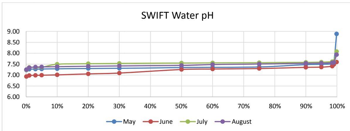
Figure 2: Distribution of Monthly SWIFT Water pH values. The infrequent high pH values are associated with continued optimization the tuning of the proportional-integral-derivative (PID) pH controller that adjusts the sodium hydroxide metering pump speed. These brief periods of elevated pH did not pose a water quality concern. Mobilization of metals within the aquifer is a concern with extended periods of low pH.
