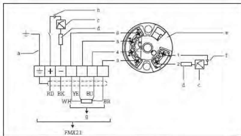
Waterpilot FMX21 with Pt100 and TMT182 temperature head transmitter (4 to 20 mA) 1) versions 'NB' and 'PT', feature 610 and 620 in the order code (→ 128)
