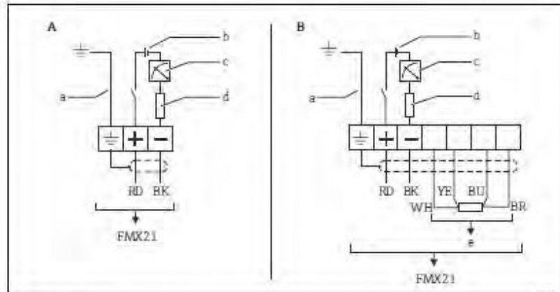
A Waterpilot FMX21 B Waterpilot FMX21 with Pt100 H-Version 1) for feature 610 'Accessories' in the order code (→ 128)
