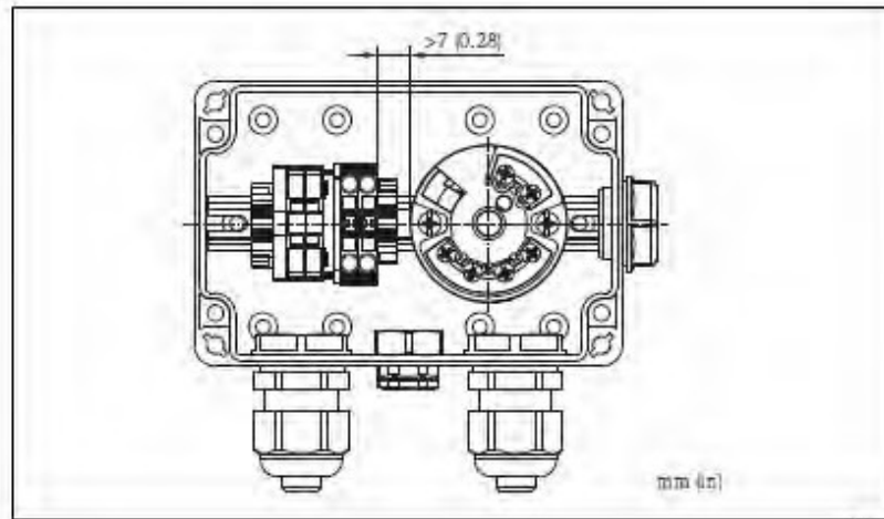
Terminal box with integrated TMT182 temperature head transmitter (4 to 20 mA HART)
