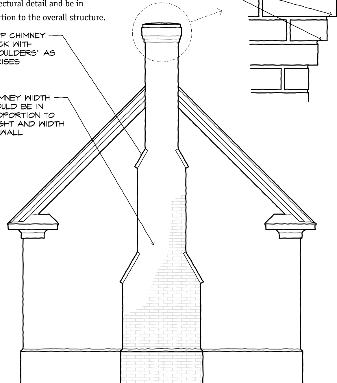
CHIMNEY ELEVATION
