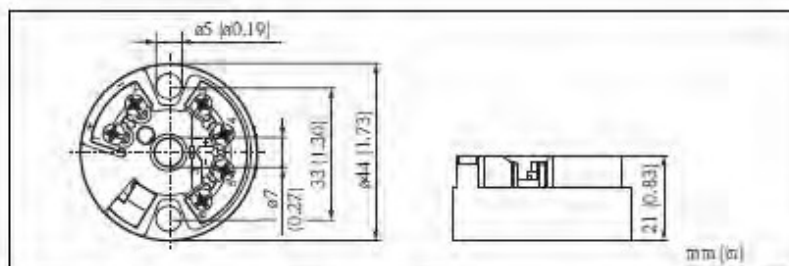
Dimensions of the TMT182 temperature head transmitter
