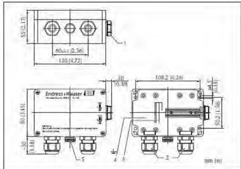
Dimensions of the IP66, IP67 terminal boxes with filters
