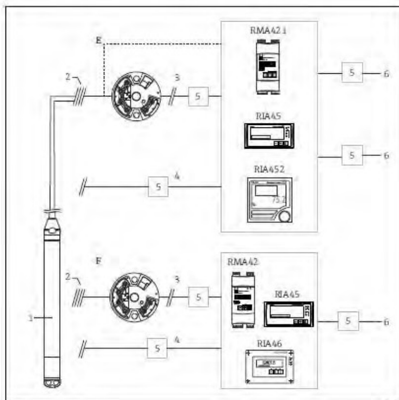
Application examples with Pt100
