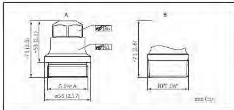
Dimensions of the extension cable mounting screws
