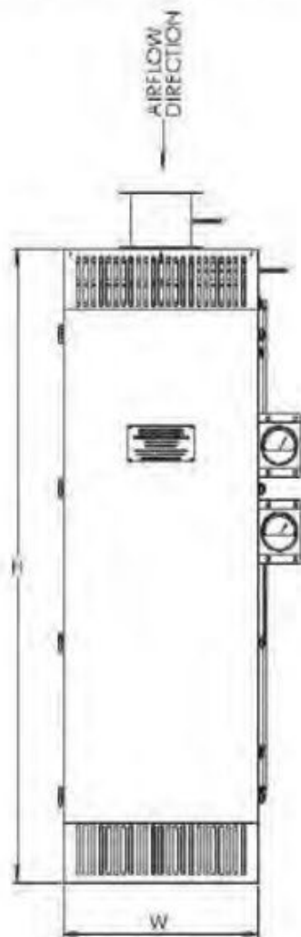
ELEVATION VIEW
