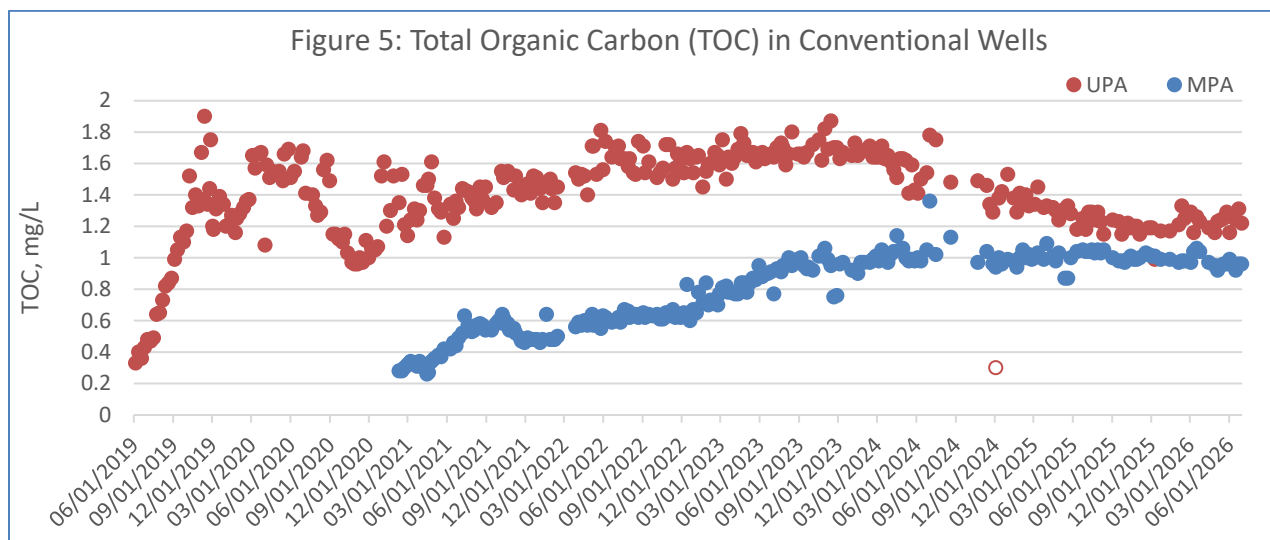
Figure 5: TOC concentration in the Upper and Middle Potomac conventional monitoring wells, MW-UPA and MW-MPA. Open circles represent data that is less than the reporting limit.
