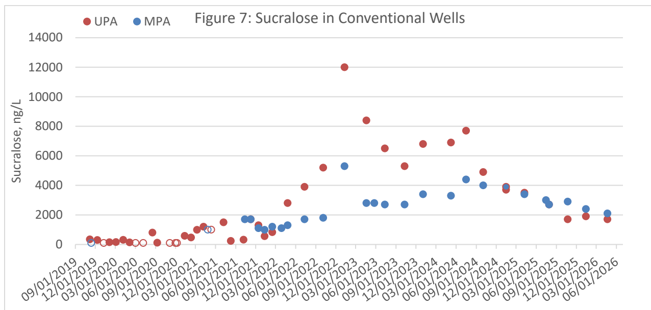
Figure 7: Sucralose trending in MW-UPA and MW-MPA. Open circles represent data that is less than the reporting limit.
