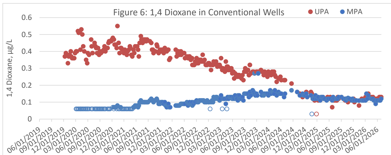
Figure 6: 1,4-Dioxane trending in MW-UPA and MW-MPA. Open circles represent data that is less than the reporting limit.
