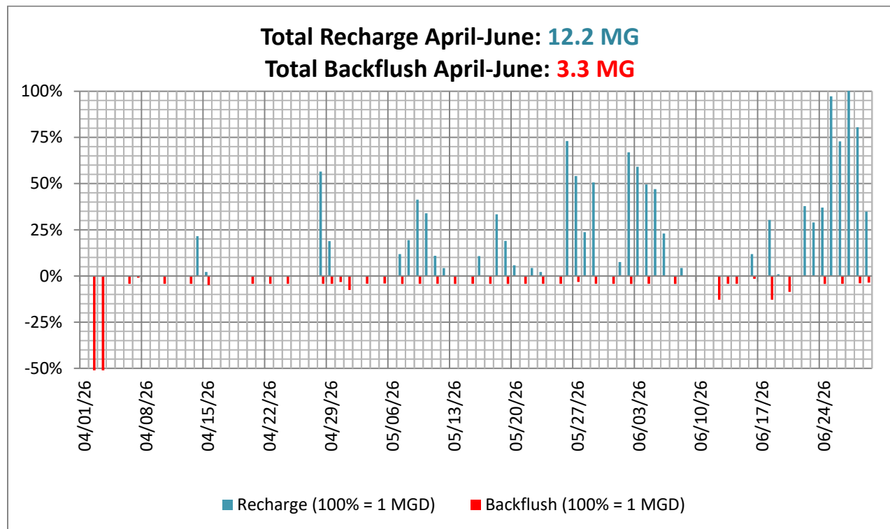
Figure 3: Recharge and Backflush Volumes, April 1 – June 30, 2026
