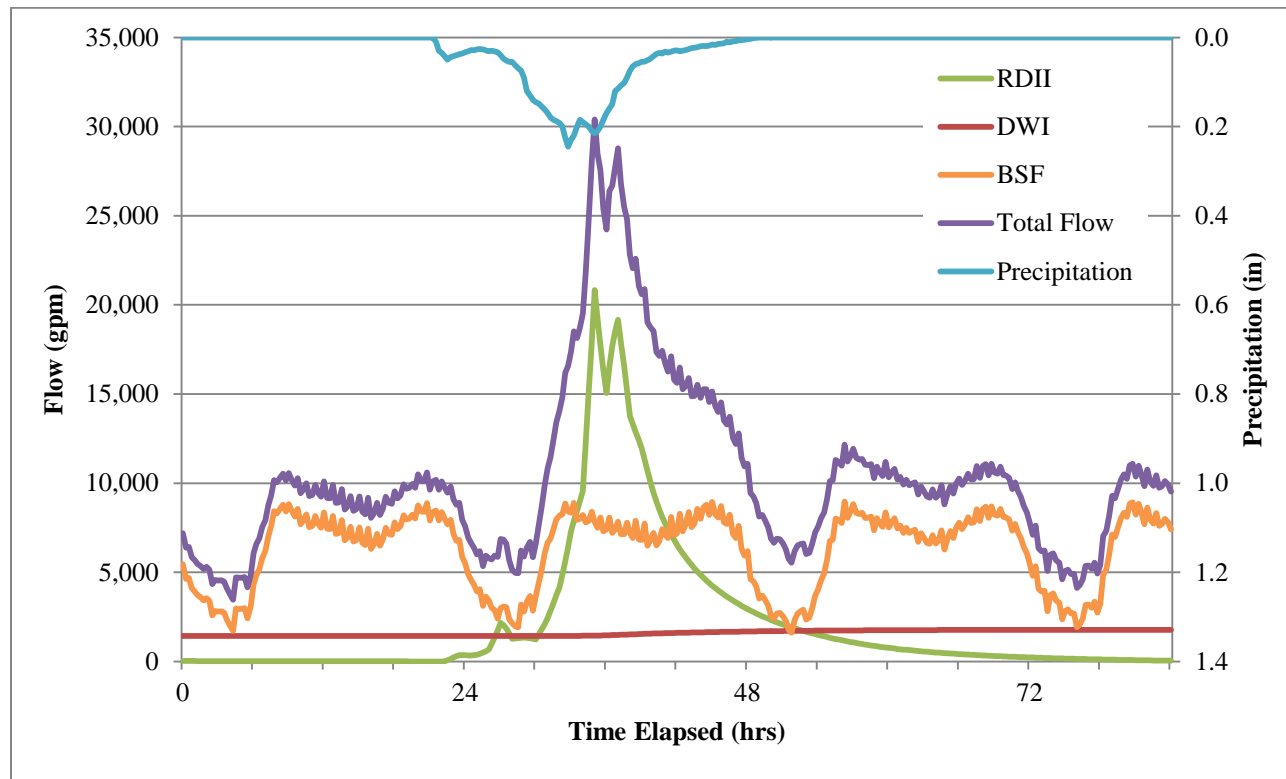
Figure 3-1. Example Components of Sewer Flow
