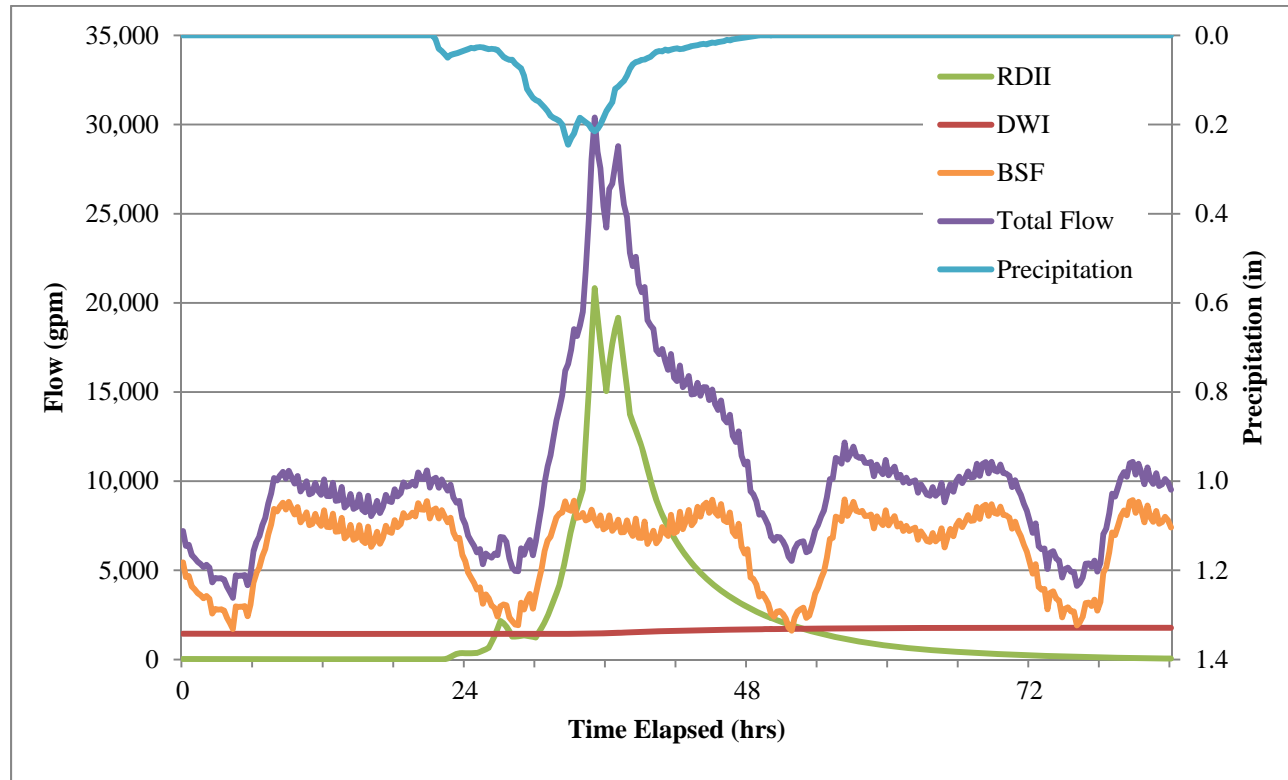
Figure 3-1. Example Components of Sewer Flow
