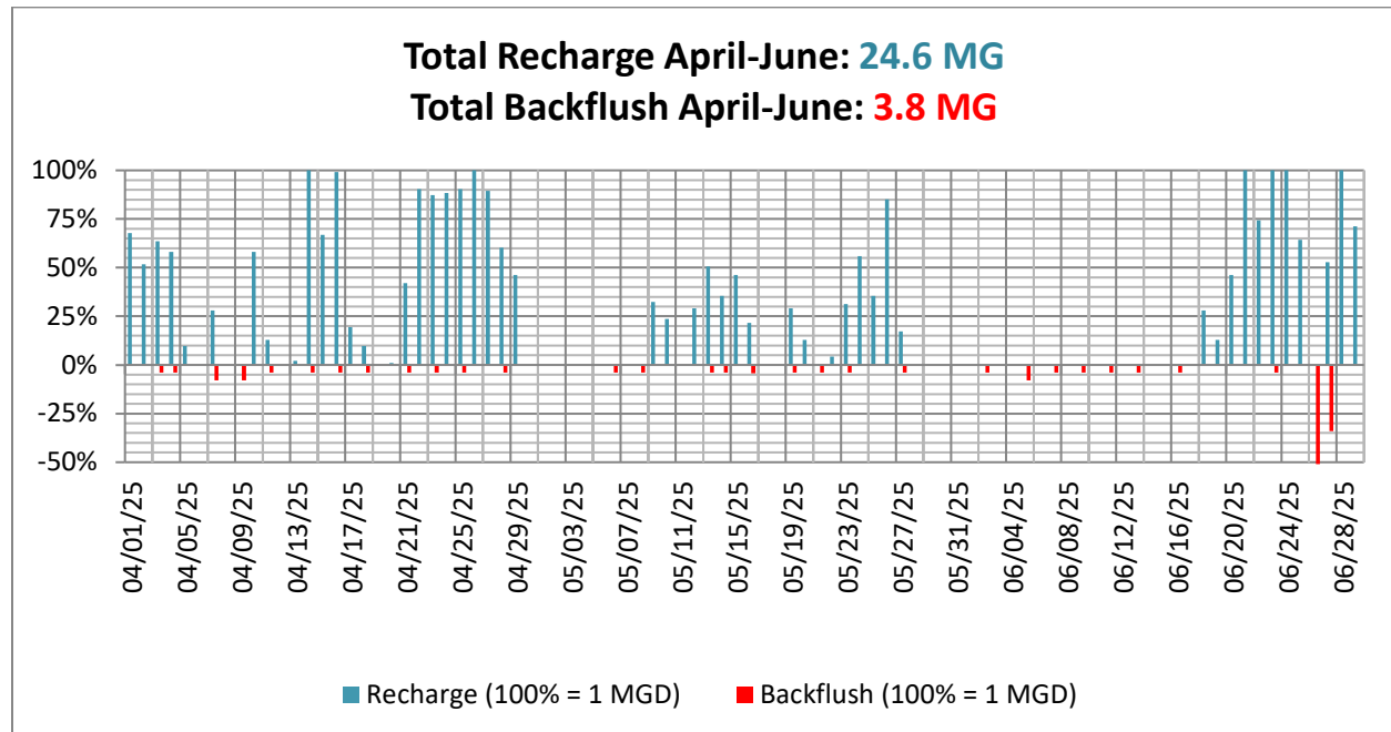
Figure 3: Recharge and Backflush Volumes, April 1 – June 30, 2025
