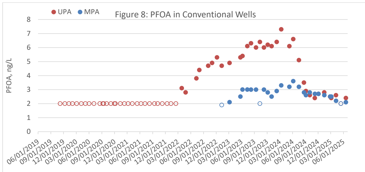
Figure 8: PFOA trending in MW-UPA. Open circles represent data that is less than the reporting limit. Based on travel time studies using a conservative tracer, SWIFT water recharged in the 1st quarter of 2023 roughly approximates the groundwater represented in this quarter's conventional well monitoring. The SWIFT water PFOA concentration for January – March 2023 was 1.1 ng/L, with a maximum value of 3.3 ng/L (n = 3). It is important to note that until July of 2022 when EPA released interim Health Advisory Limits (HAL) for PFOA and PFOS, HRSD's operational controls for these compounds were based upon the previous HAL of 70 ng/L FOA+PFOS. Since that time, HRSD has optimized GAC performance to maintain PFOA and PFOS below 4 ng/L.
