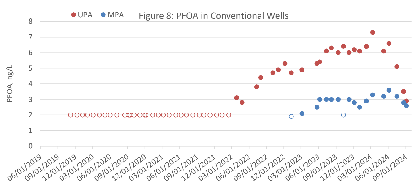
Figure 8: PFOA trending in MW-UPA. Open circles represent data that is less than the reporting limit. Based on travel time studies using a conservative tracer, SWIFT water recharged in the 3rd quarter of 2022 roughly approximates the groundwater represented in this quarter's conventional well monitoring. The SWIFT water PFOA concentration for July - September 2022 was 11.2 ng/L, with a maximum value of 13.0 ng/L (n = 3). It is important to note that until July of 2022 when EPA released interim Health Advisory Limits (HAL) for PFOA and PFOS, HRSD's operational controls for these compounds were based upon the previous HAL of 70 ng/L FOA+PFOS. Since that time, HRSD has been working to optimize GAC performance to maintain PFOA and PFOS below 4 ng/L.
