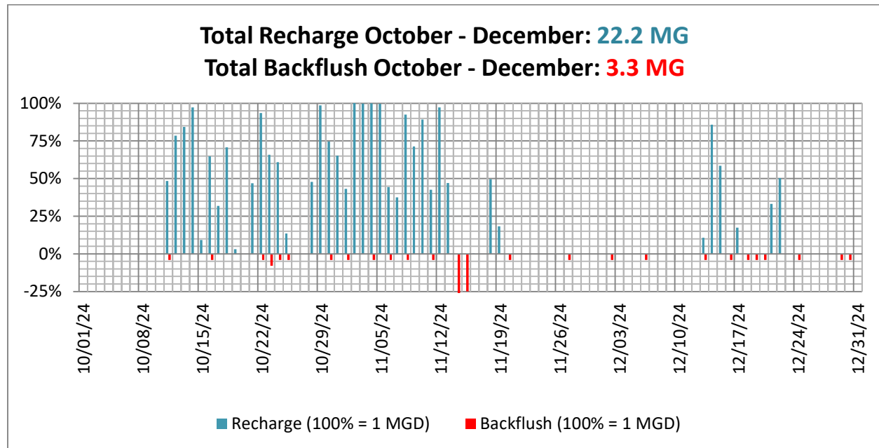
Figure 3: Recharge and Backflush Volumes, October 1 – December 31, 2024
