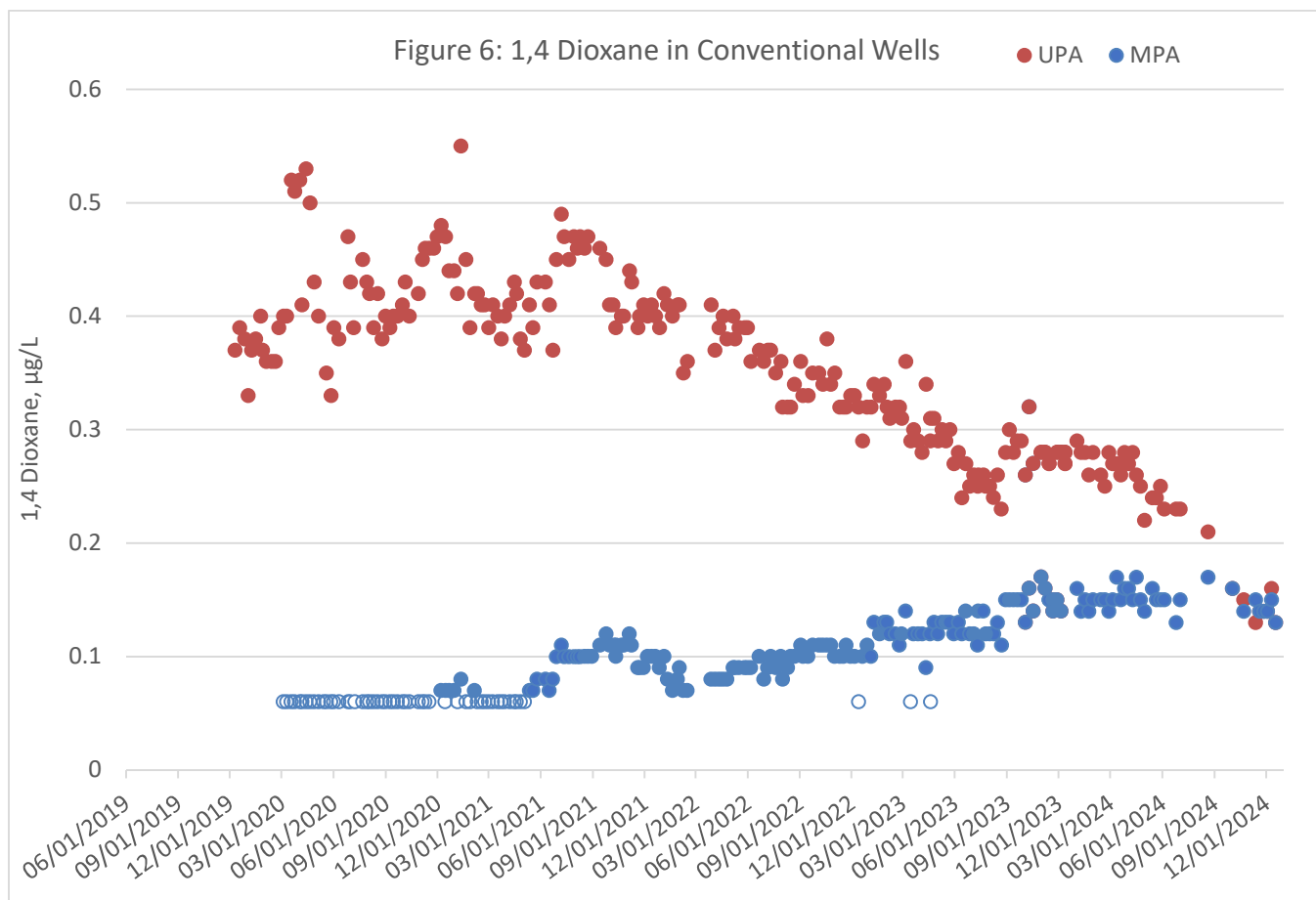
Figure 6: 1,4-Dioxane trending in MW-UPA and MW-MPA. Open circles represent data that is less than the reporting limit. Based on travel time studies using a conservative tracer, SWIFT water recharged in the 4th quarter of 2022 roughly approximates the groundwater represented in this quarter's conventional well monitoring. The SWIFT water average 1,4-dioxane concentration for October - December 2022 was 0.16 µg/L, with a maximum value of 0.19 µg/L (n = 12).
