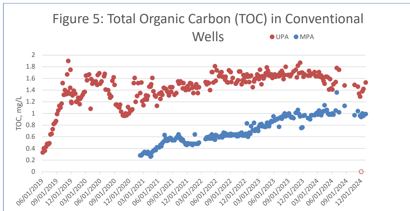
Figure 5: TOC concentration in the Upper and Middle Potomac conventional monitoring wells, MW-UPA and MW-MPA. Open circles represent data that is less than the reporting limit. Based on travel time studies using a conservative tracer, SWIFT water recharged in the 4th quarter of 2022 roughly approximates the groundwater represented in this quarter's conventional well monitoring. The SWIFT water average TOC concentration for October - December 2022 was 2.36 mg/L, with a maximum of 3.01 mg/L (n = 43).
