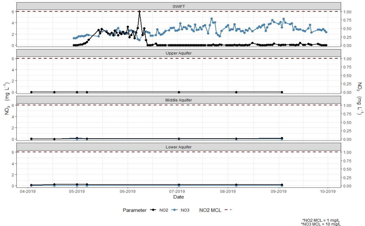
Figure 6: Average Daily Nitrite Concentration in the conventional monitoring wells (MW-UPA, MW-MPA, MW-LPA).
