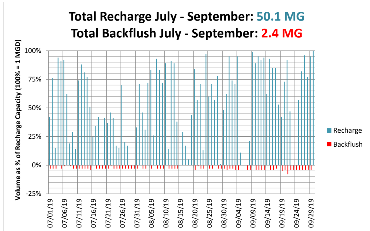
Figure 3: Recharge and Backflush Volumes, July 1 – September 30, 2019.
